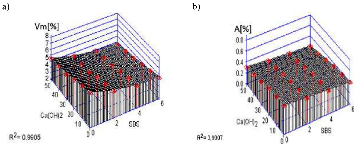
Figure 1 : The influence of hydrated lime ( Ca(OH)_2 ) and polymer (SBS) on a) void contents ( V_m ), b) water absorption (A) of SMA asphalt
