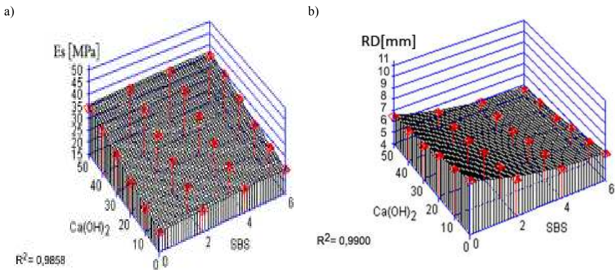
Figure 2 : The influence of hydrated lime ( Ca(OH)_2 ) and polymer content (SBS) on a) static creep modulus ( E_s ) and b) rut depth (RD) of SMA
