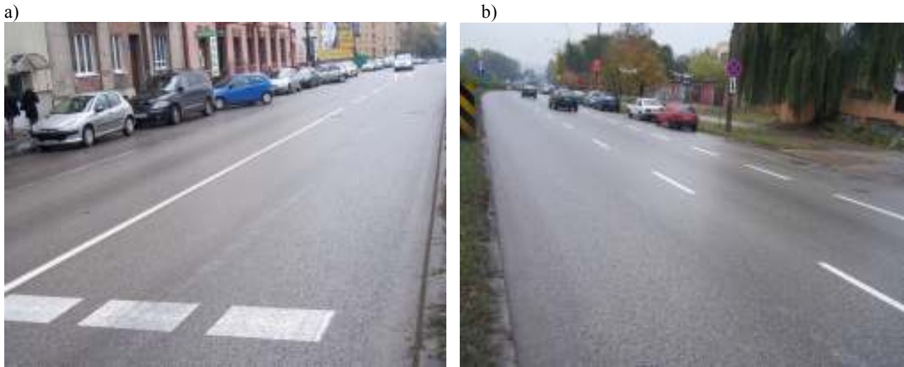
Figure 5 : View of surface of SMA after 12 years operation depending on type of adhesion agent a) hydrated lime, b) fatty amine
